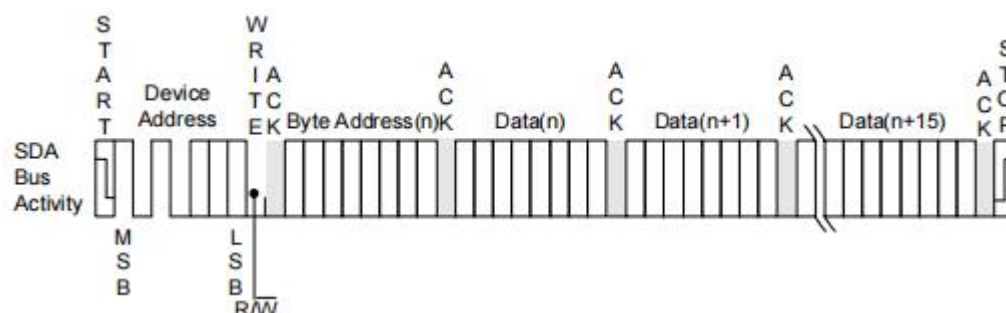
Figure 7. Page Write
