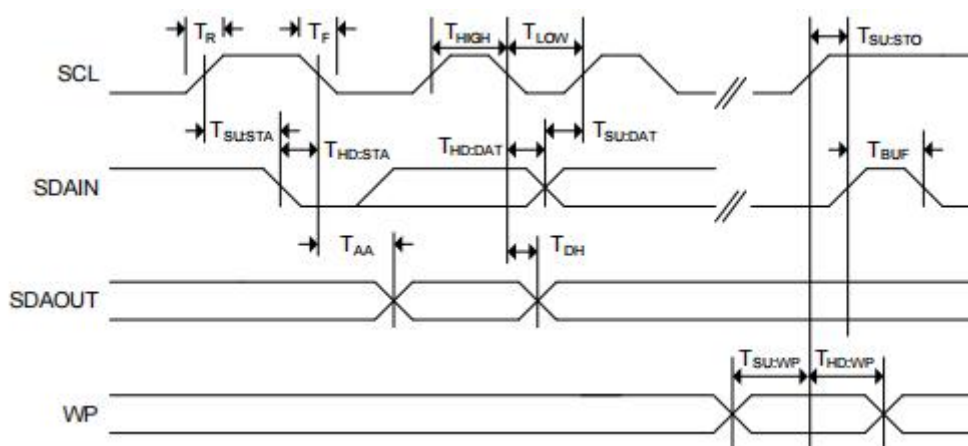
Figure 11. Bus Timing
