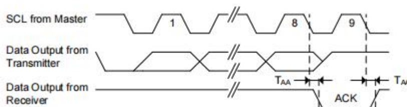
Figure4.Output Acknowledge
