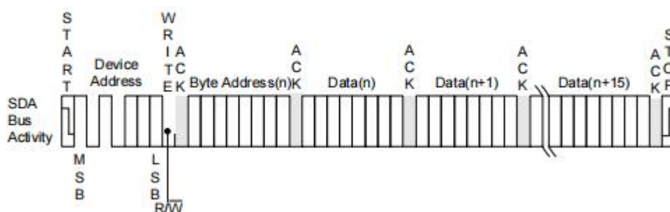
Figure 7. Page Write
