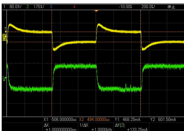
Fig 9. Load Transient (1mA to 300mA)
