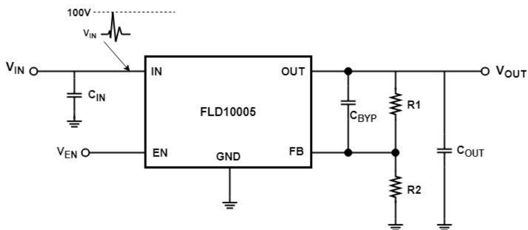
Figure 4. Typical Application for FLD10005
