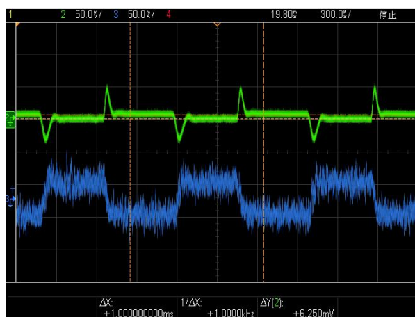
Fig 5. Load transient 0 to 50mA
