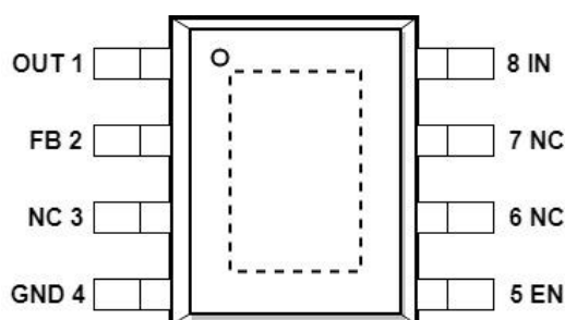
Figure 1. Pin Assignment of FLD10005 Package ESOP8
