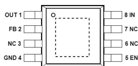
Figure 3. Pin Assignment of FLD10005 Package MSOP8
