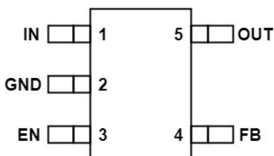
Figure 2. Pin Assignment of FLD10005 Package SOT23-5
