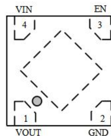
DFN1x1-4
