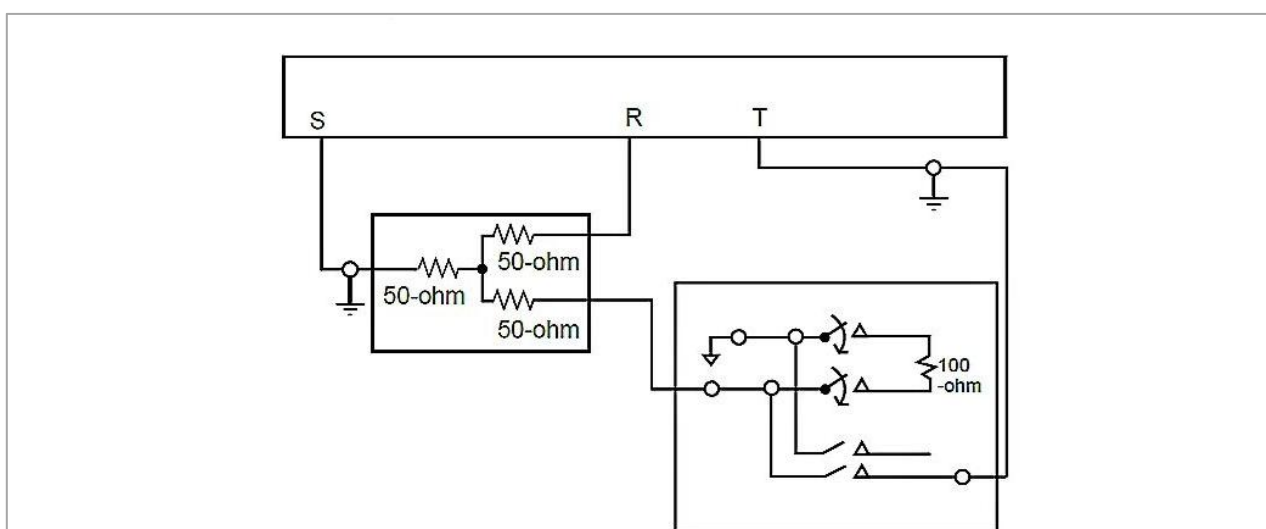
Fig.2 OFF-isolation
