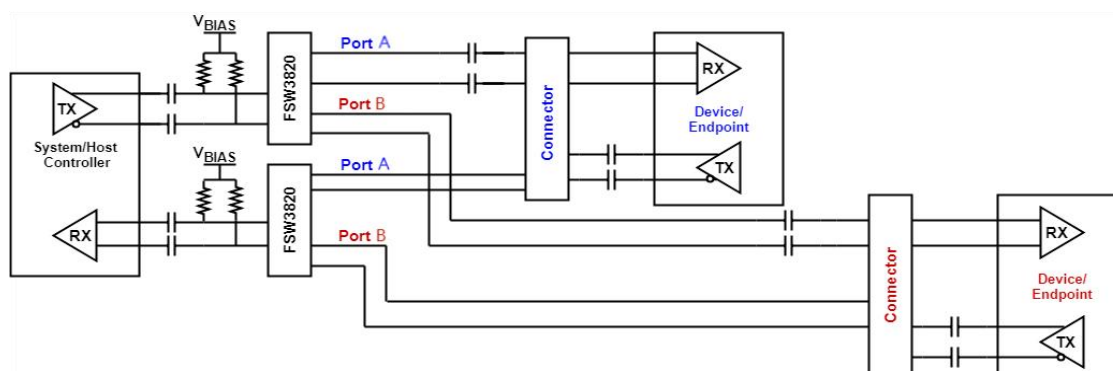
Figure 3. AC Coupling Capacitors on Both Sides of Switch
