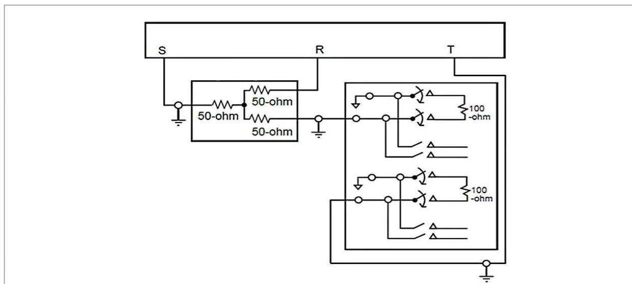
Fig.1 Crosstalk Setup
