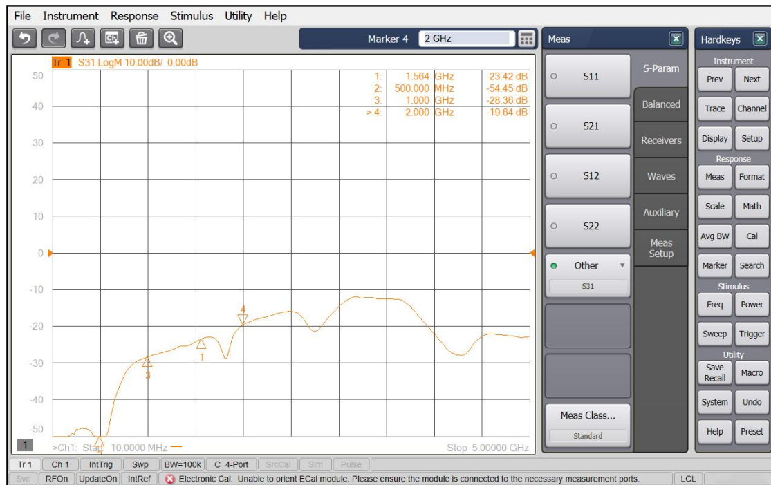
Fig 8. Switch Cross-Talk
