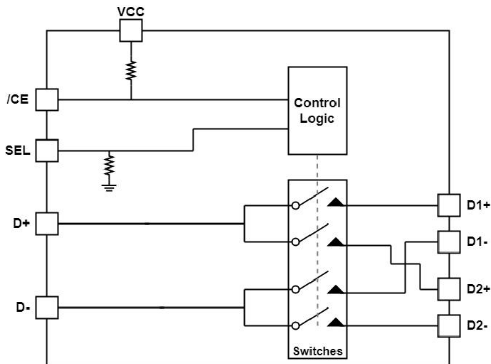
Figure 5. Internal function diagram
