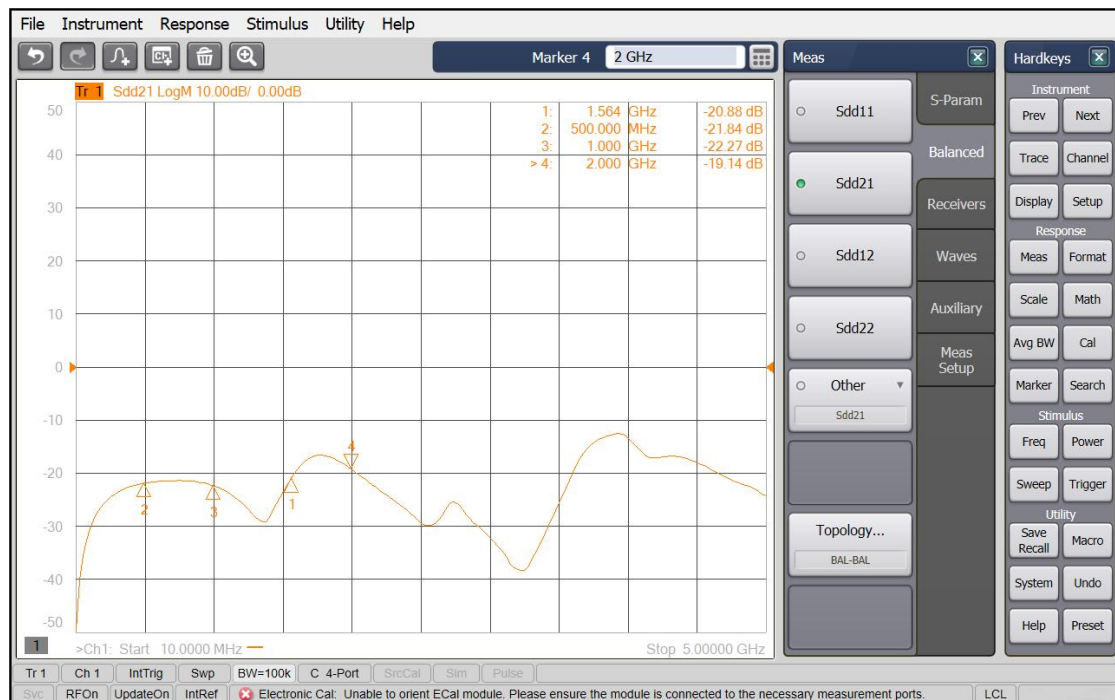
Fig 9. Switch Off Isolation
