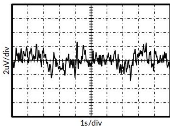
Figure 9. 0.1Hz to 10Hz Input Voltage Noise
