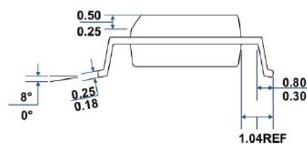
LEFT-SIDE VIEW
