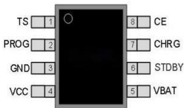
ESOP8 TOP VIEW
