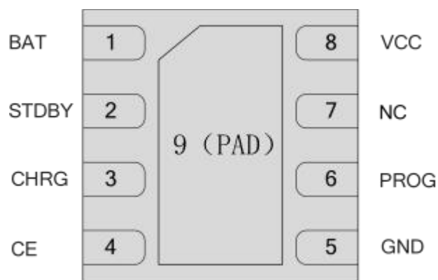
DFN3×3_8L
