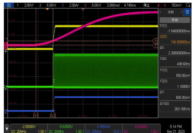
Fig 8 Enable Start up ( V_{in}=12V , V_{out}=3.3V , I_{LOAD}=2A )
