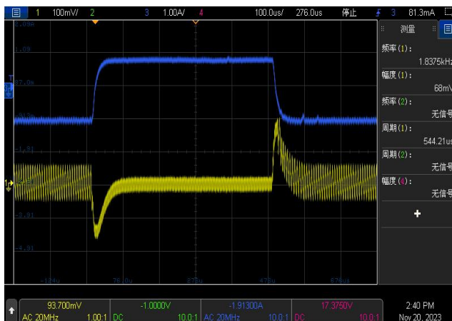
Fig 7 Load Transient ( V_{in}=12V , V_{out}=3.3V , I_{LOAD}=0.2-2A )
