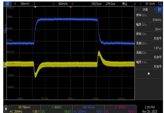
Fig 6 Load Transient ( V_{in}=12V , V_{out}=3.3V , I_{LOAD}=1-2A )
