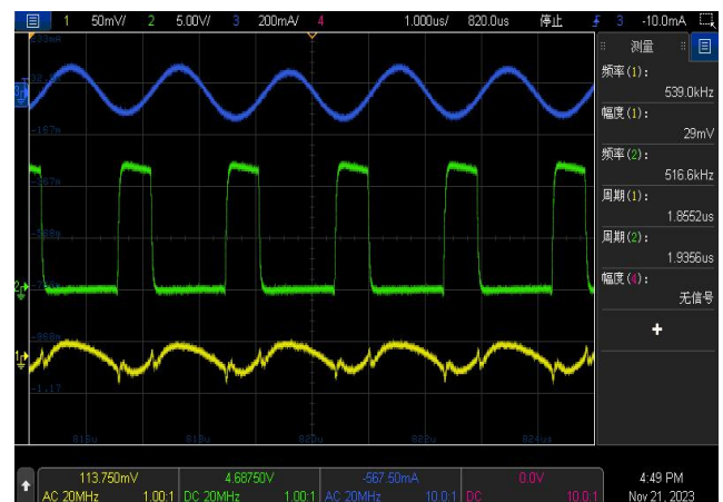
Fig 10 Output Ripple ( V_{in}=12V , V_{out}=3.3V , I_{LOAD}=2A )
