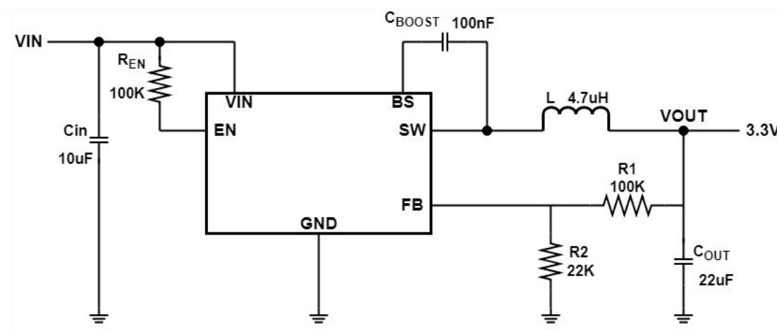
Figure 1. Typical Application for FDK1620
