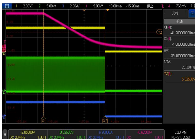
Fig 9 Shutdown ( V_{in}=12V , V_{out}=3.3V , I_{LOAD}=2A )
