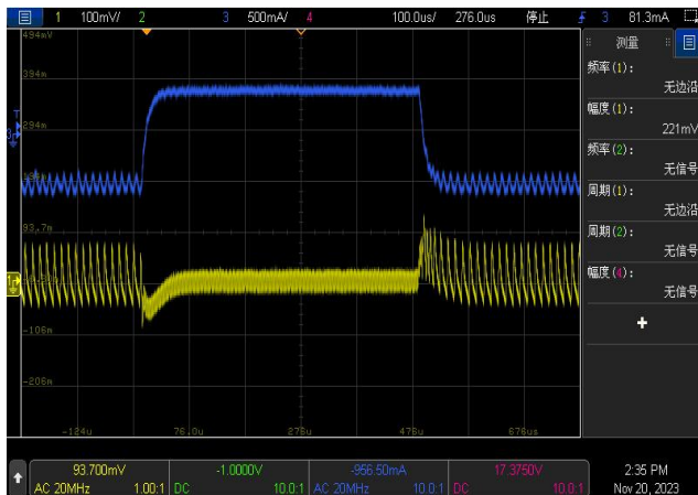
Fig 5 Load Transient ( V_{in}=12V , V_{out}=3.3V , I_{LOAD}=0.1-1A )
