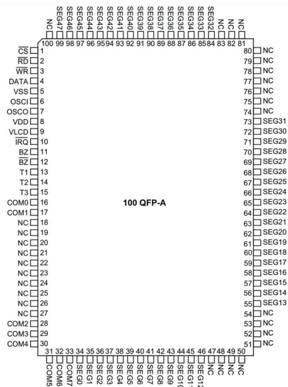
Package:QFP100
