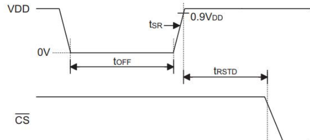
Figure 4 Power-on Reset Timing
