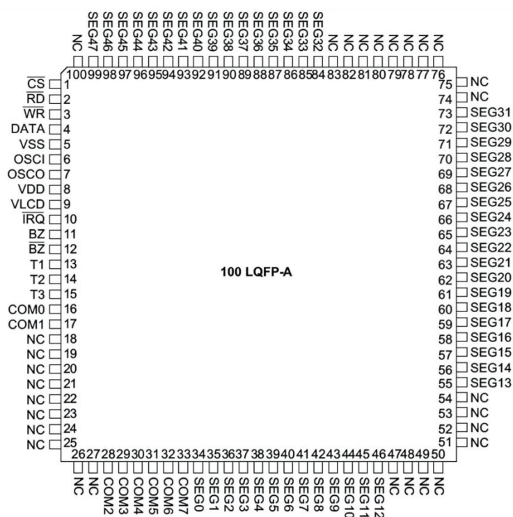
Package:LQFP100
