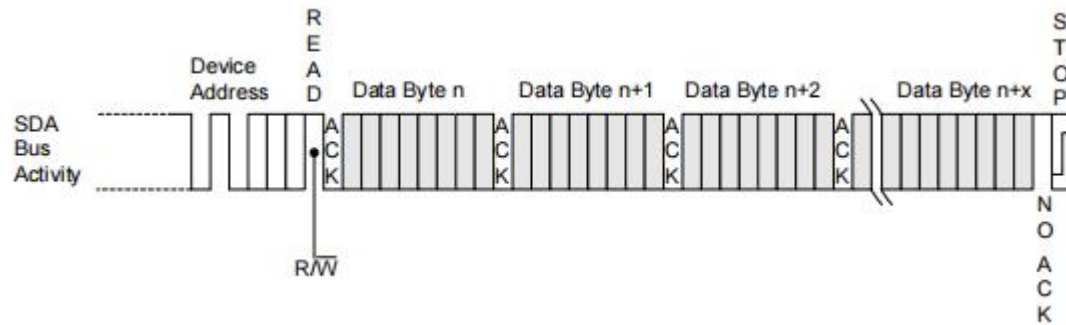
Figure 10. Sequential Read
