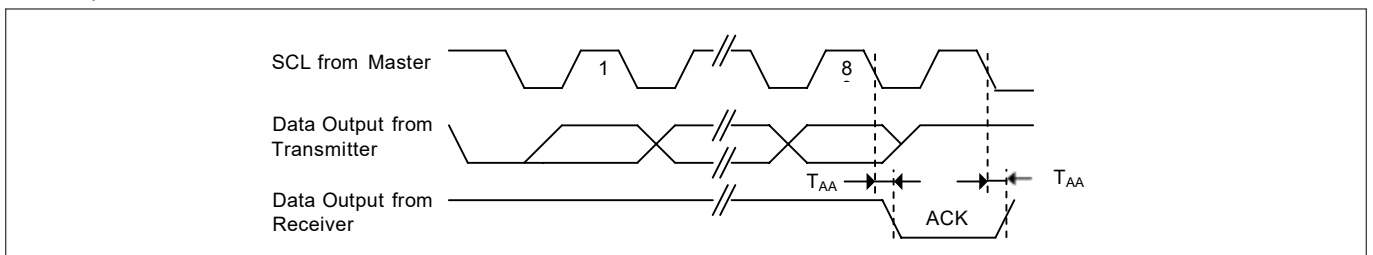
Figure4.Output Acknowledge
