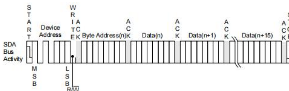
Figure 7. Page Write
