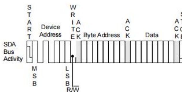
Figure 6.Byte Write
