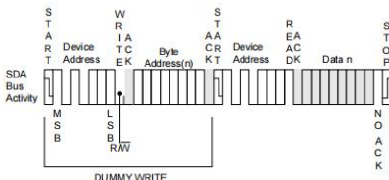
Figure 10. Sequential Read
