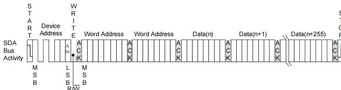
Figure 7.Page Write
