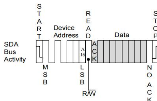
Figure8.Current Address Read
