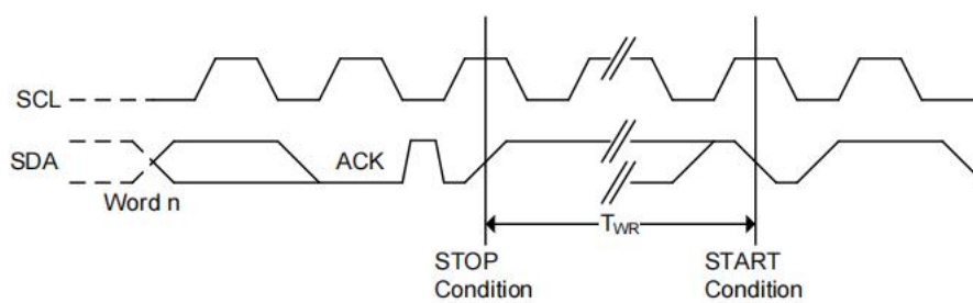
Figure 11. Bus Timing
