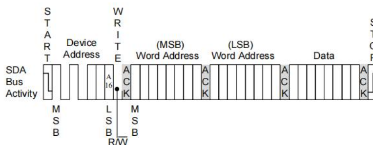
Figure6.Byte Write
