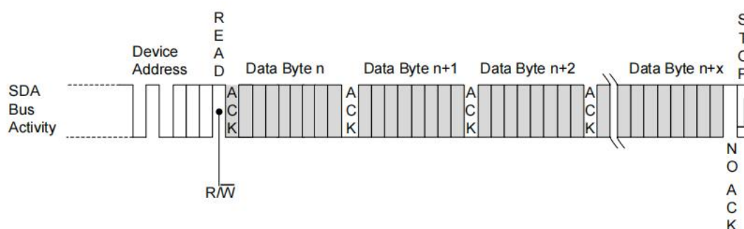
Figure 10. Sequential Read
