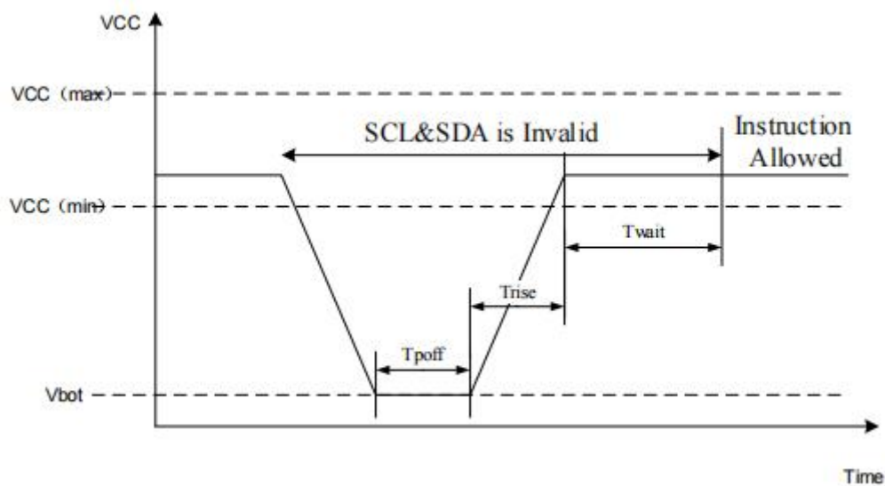
Power down-up Timing
