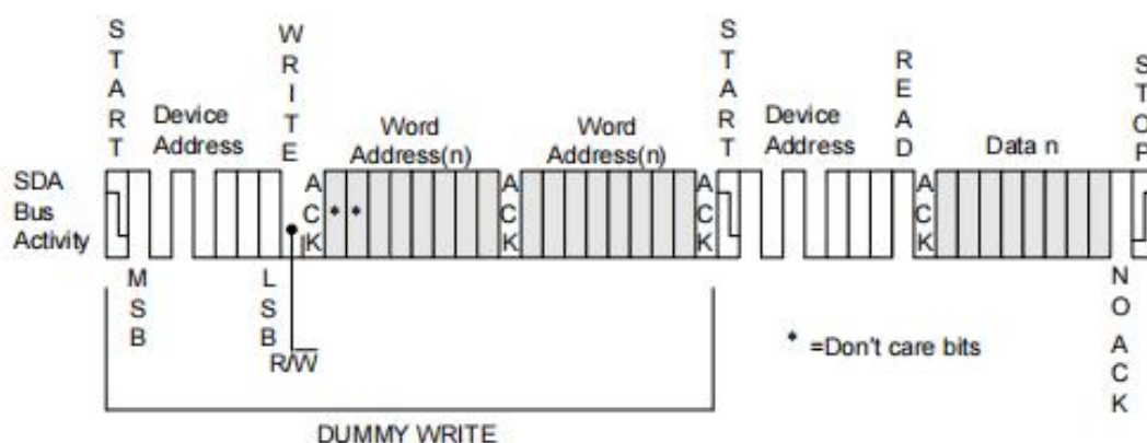
Figure 9. Random Address Read
