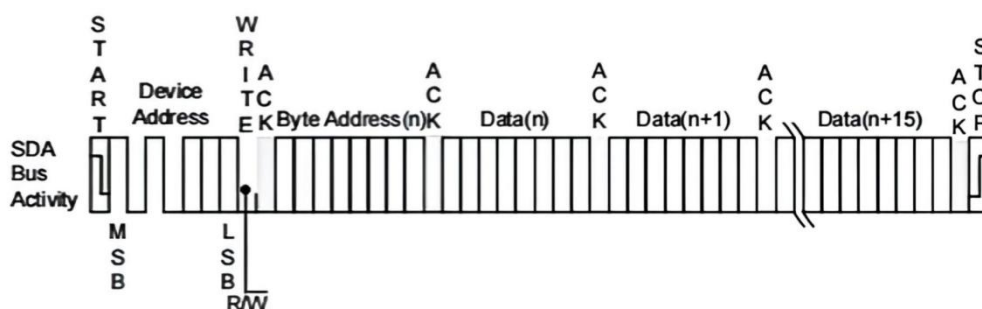
Figure 7. Page Write
