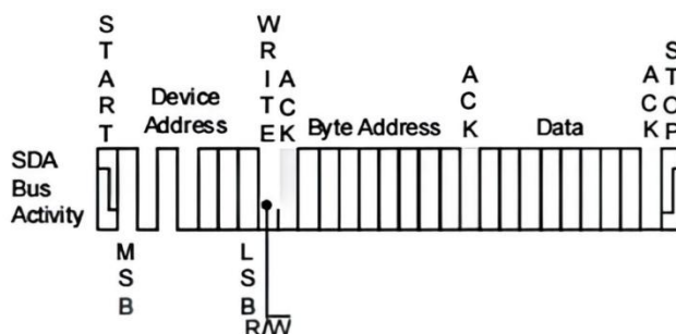
Figure 6.Byte Write
