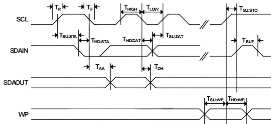
Figure 11. Bus Timing
