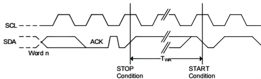
Figure 12. Write Cycle Timin
