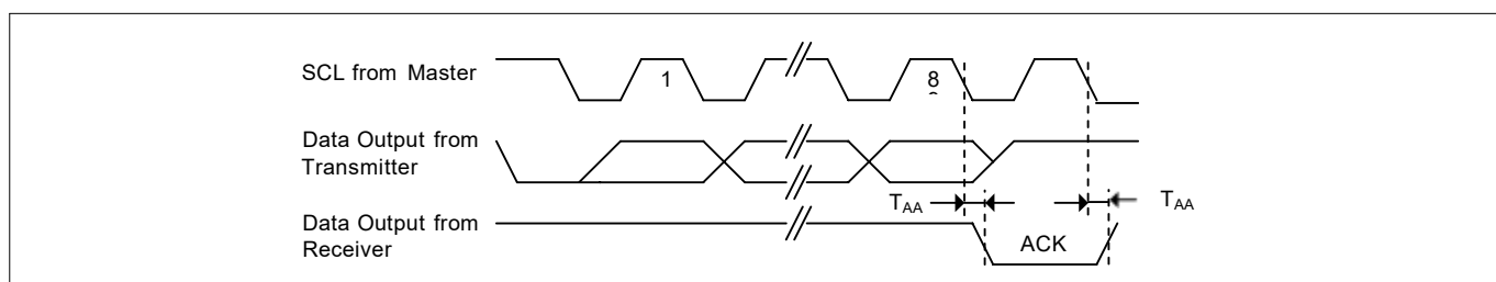
Figure4.Output Acknowledge
