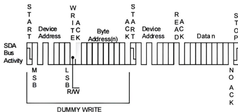
Figure 10.Sequential Read
