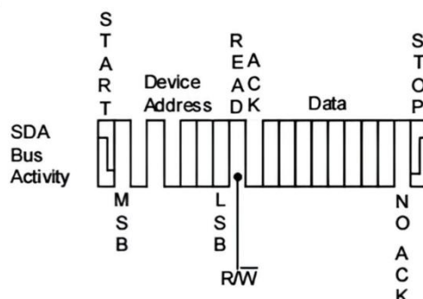
Figure8.Current Address Read
