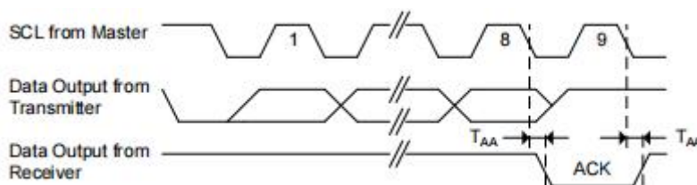
Figure 4.Output Acknowledge
