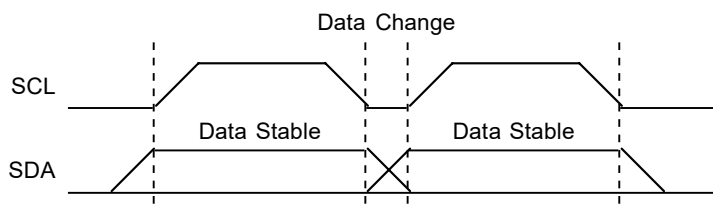
Figure 2. Data Validity Protocol
