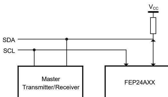
Figure 1. Typical System Bus Configuration
