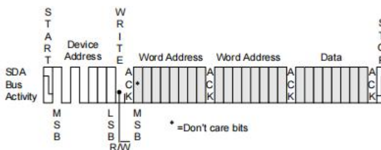
Figure 6.Byte Write
