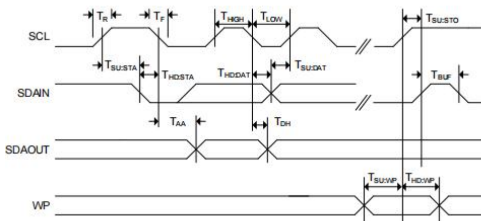
Figure 11. Bus Timing
