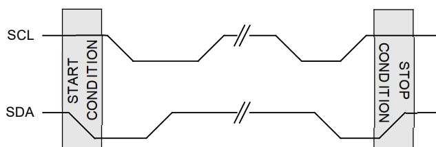
Figure3.Start and Stop Conditions
