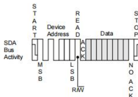
Figure8.Current Address Read
