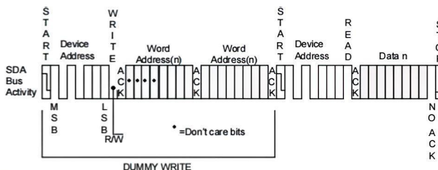
Figure9. Random Address Read
