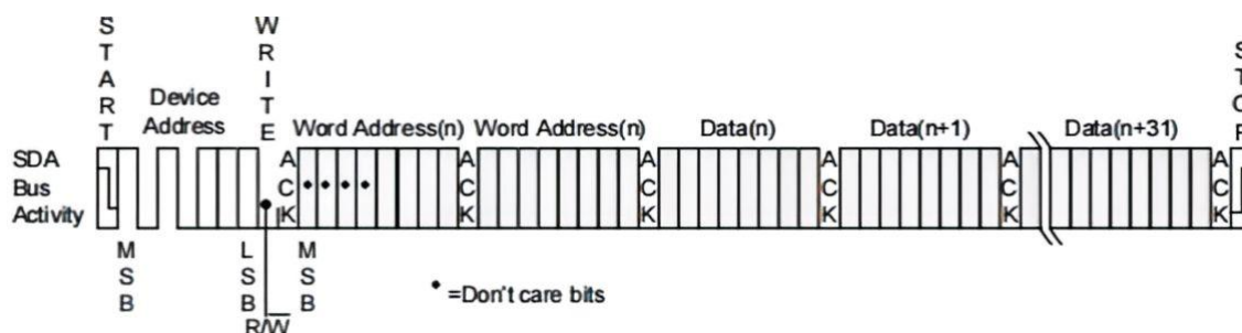
Figure 7. Page Write
