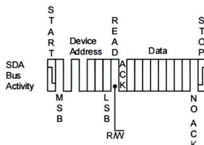
Figure8.Current Address Read
