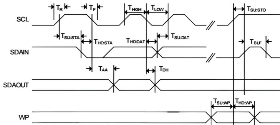
Figure 11. Bus Timing
