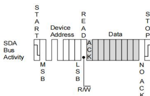
Figure8.Current Address Read
