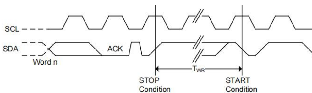
Figure 12. Write Cycle Timing
