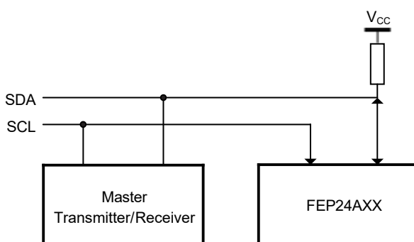
Figure 1. Typical System Bus Configuration
