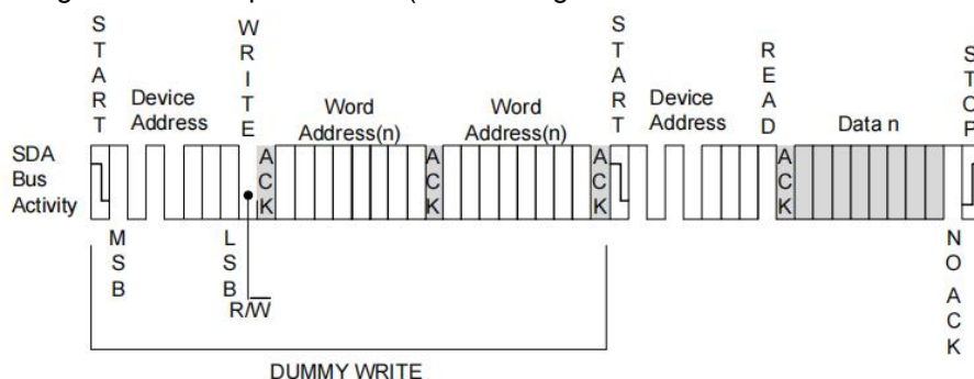
Figure9. Random Address Read
