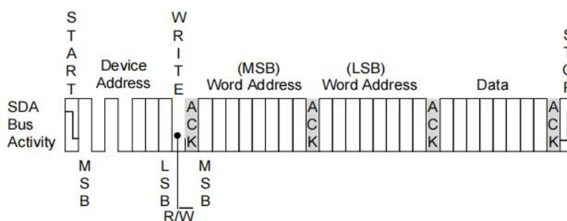
Figure6.Byte Write
