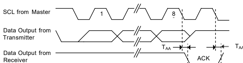
Figure4.Output Acknowledge
