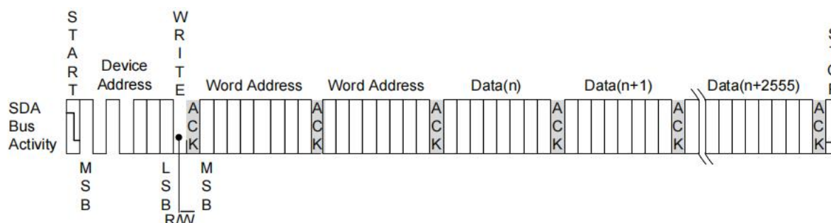
Figure 7.Page Write
