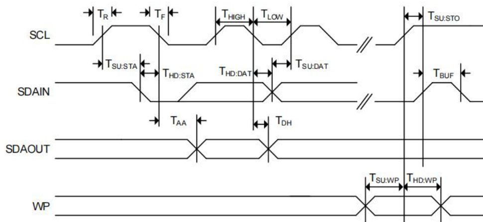
Figure 11. Bus Timing
